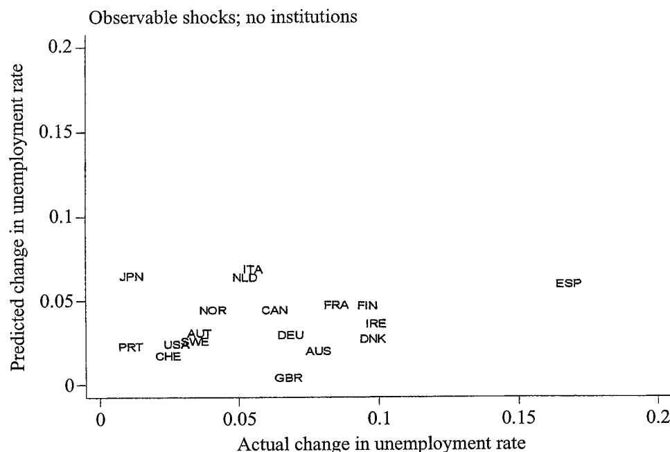
Fig. 10. Actual and Predicted Change in u, 1965–9 to 1990–4
