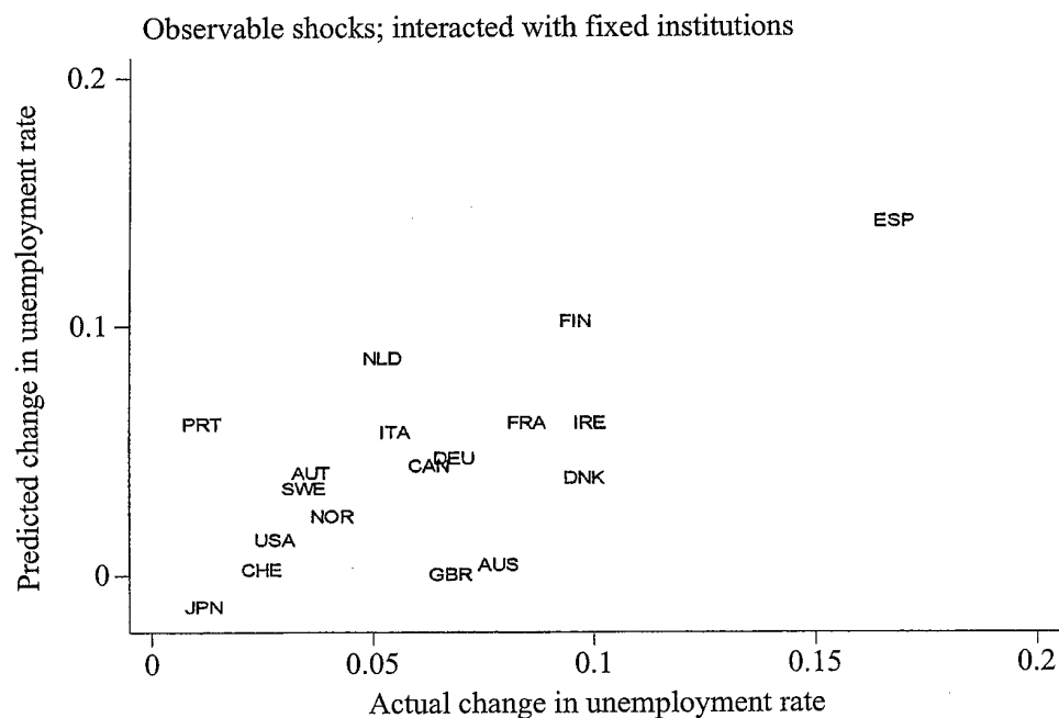
Fig. 11. Actual and Predicted Change in u, 1965–9 to 1990–4
