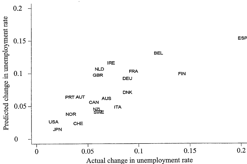
Fig. 9. Actual and Predicted Change in u , 1995+ over 1965–9
